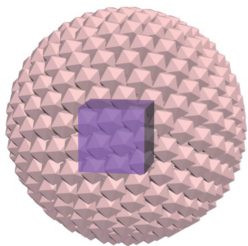
Core-shell structure
