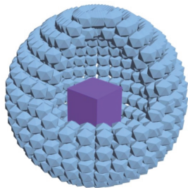
Yolk-shell structure
