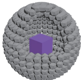
Yolk-shell structure
